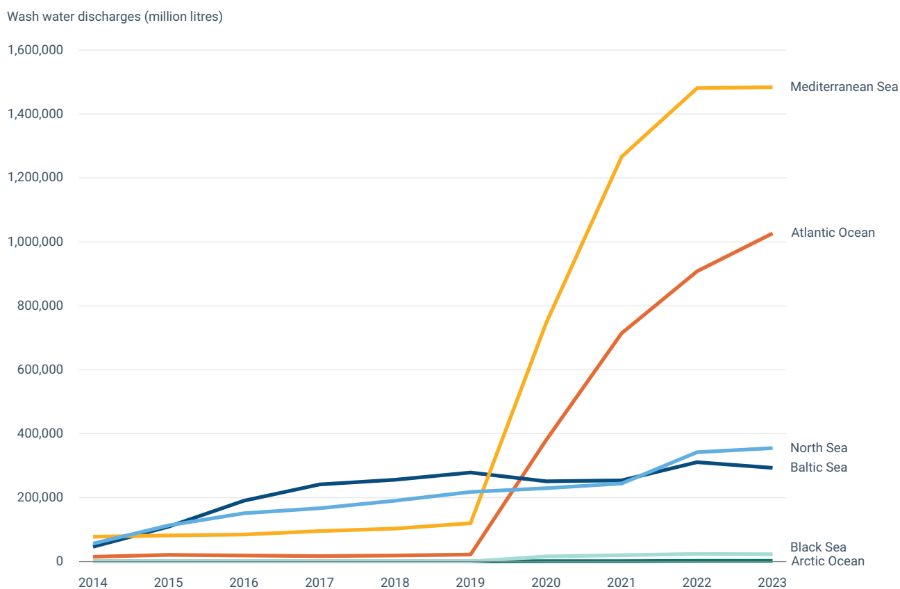
Figure 2.29 Wash water discharges from open loop scrubbers per region in EU waters
