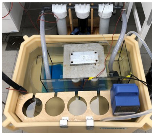
Figure 14. Set up for the controlled temperature of holding tank for ISO 15181-1 using a water bath.
