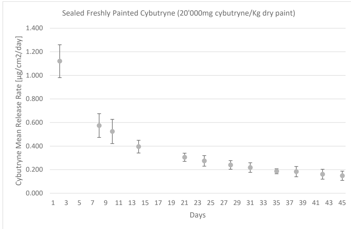
Figure 17 the plot shows the mean release rate of cybutryne for the “Sealed Freshly painted Cybutryne coatings (20’000mg Cybutryne/Kg dry paint)” during the 45 days of the study. Mean release rates values are plotted as a function of time.
