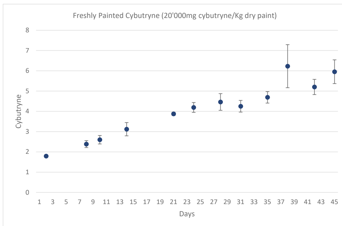
Figure 16 - The plot shows the mean release rate of cybutryne for the “ Freshly painted Cybutryne coatings (20'000 mg Cybutryne/Kg dry paint) ” during the 45 days of the study. Mean release rates values are plotted as a function of time.
