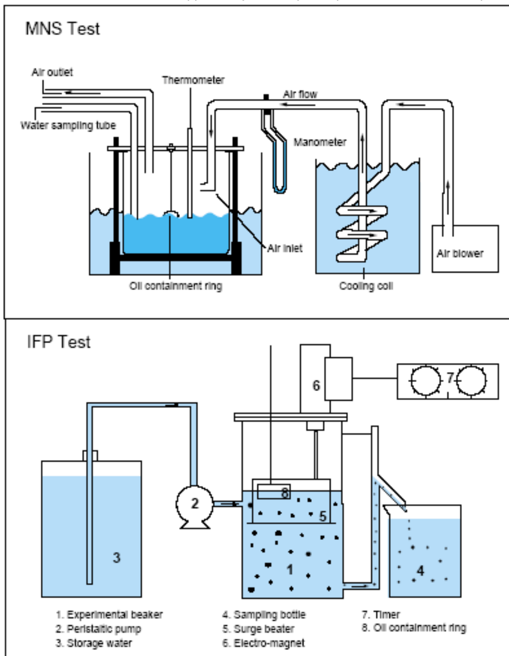
Figure 6. The MNS and IFP dispersant test methods
