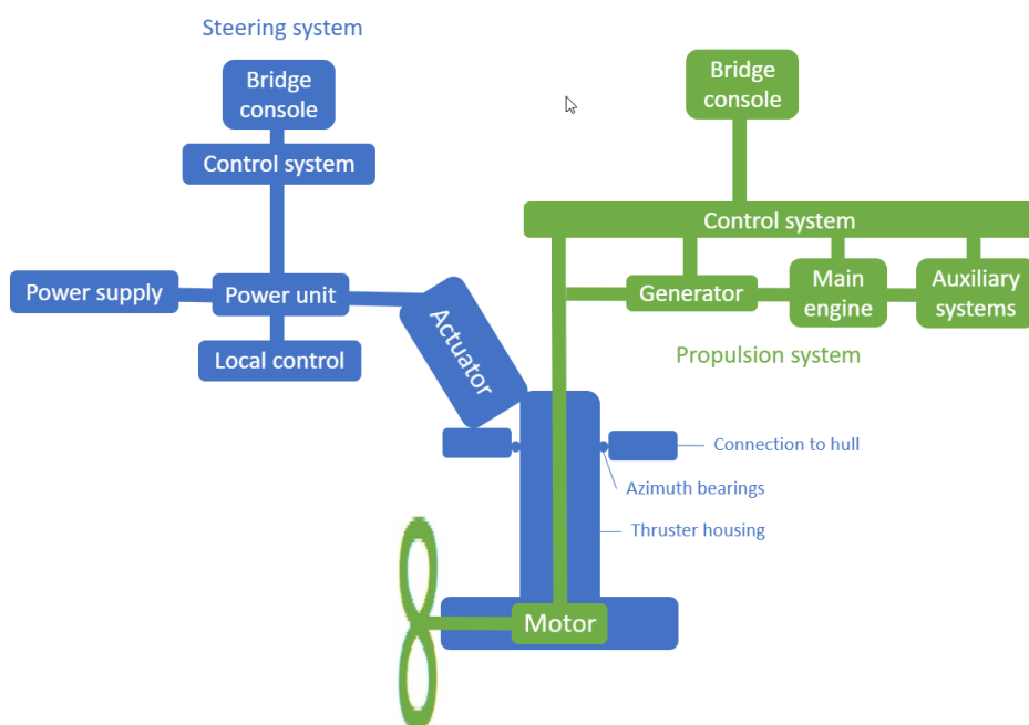
Figure 5-3 Podded propulsion system
