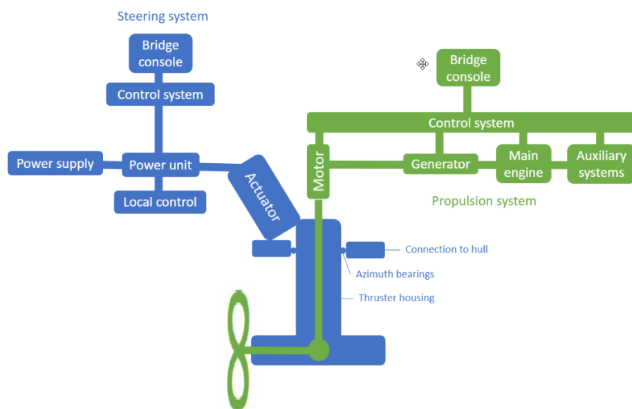
Figure 5-2 Azimuth system
