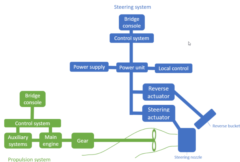
Figure 5-4 Waterjet system
