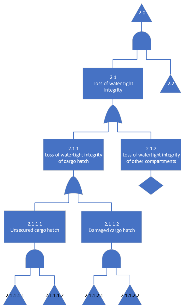
Figure 30 – Fault tree branches for intermediate event ID 2.1
