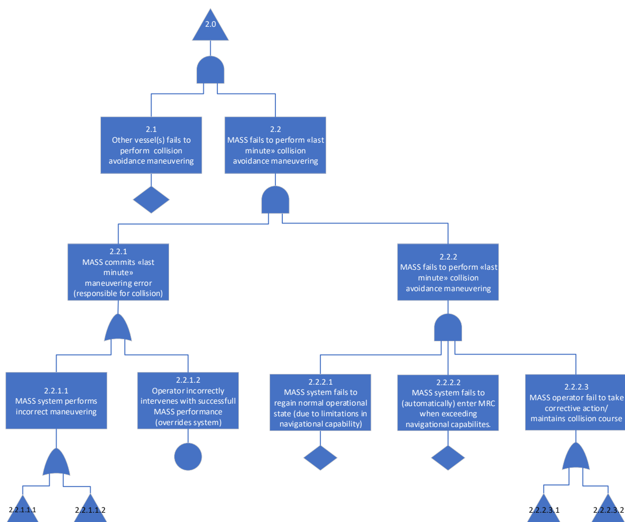
Figure 23 – Fault tree branches for intermediate event ID 2.0
