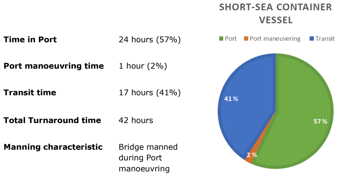
Figure 12 – Operational profile for a Container feeder ship
