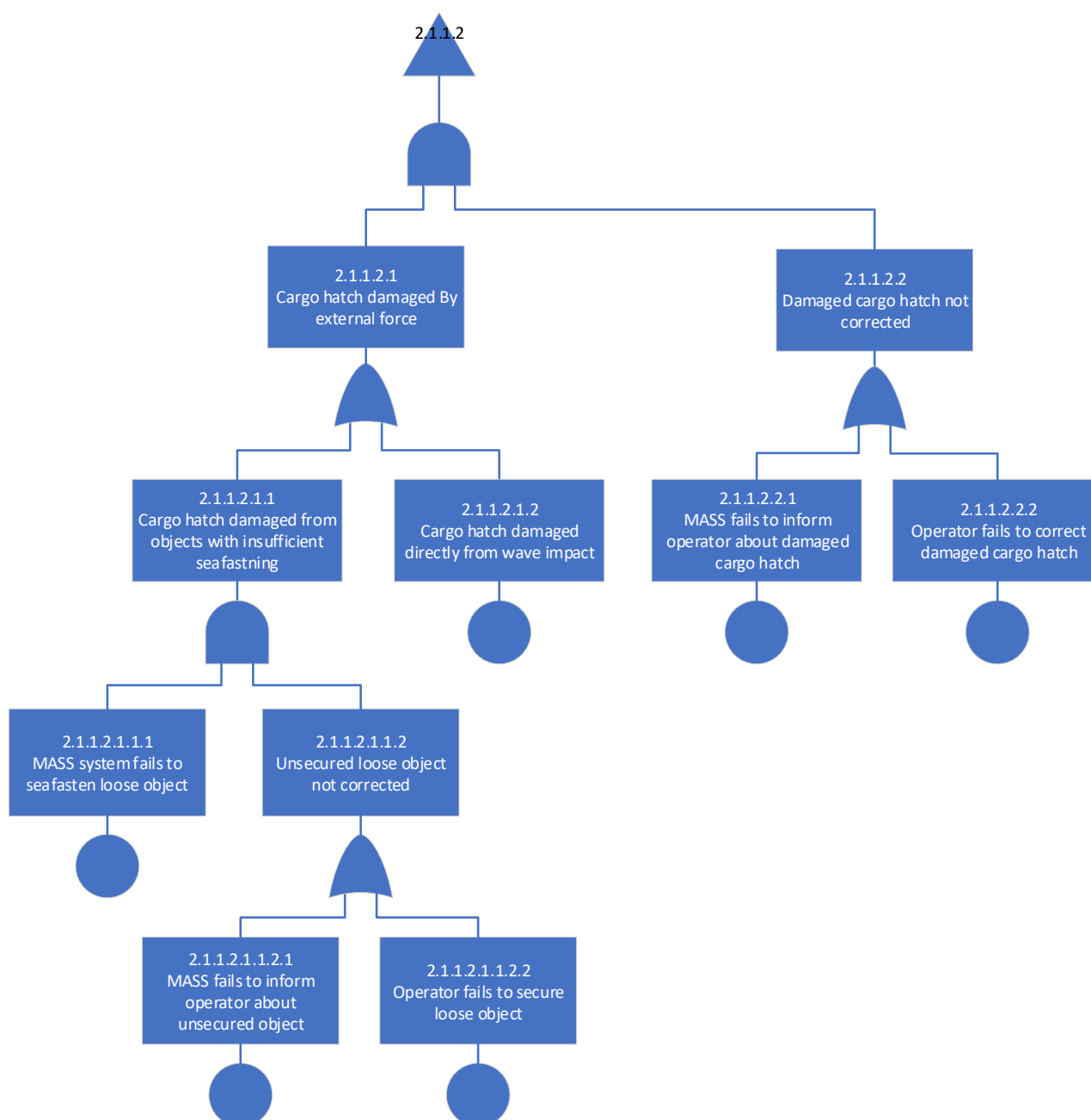
Figure 32 – Fault tree branches for intermediate event ID 2.1.1.2
